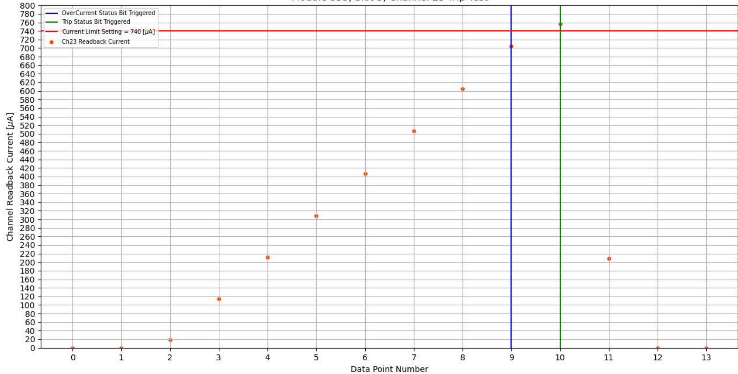
Module 355, Slot 5, Channel 23 Trip Test
