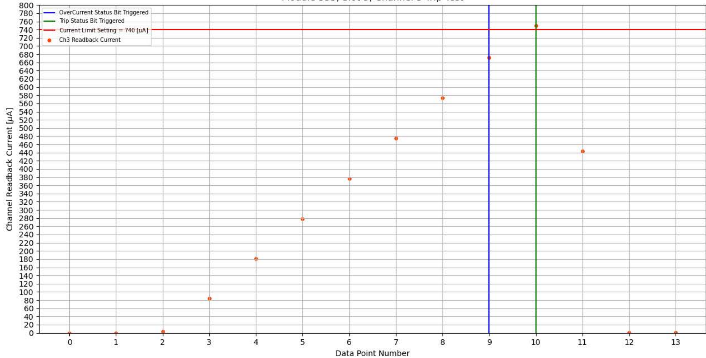
Module 355, Slot 5, Channel 3 Trip Test
