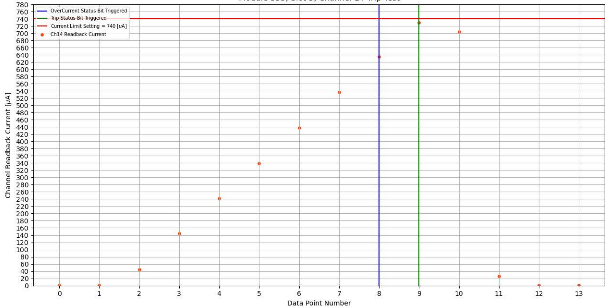
Module 355, Slot 5, Channel 14 Trip Test
