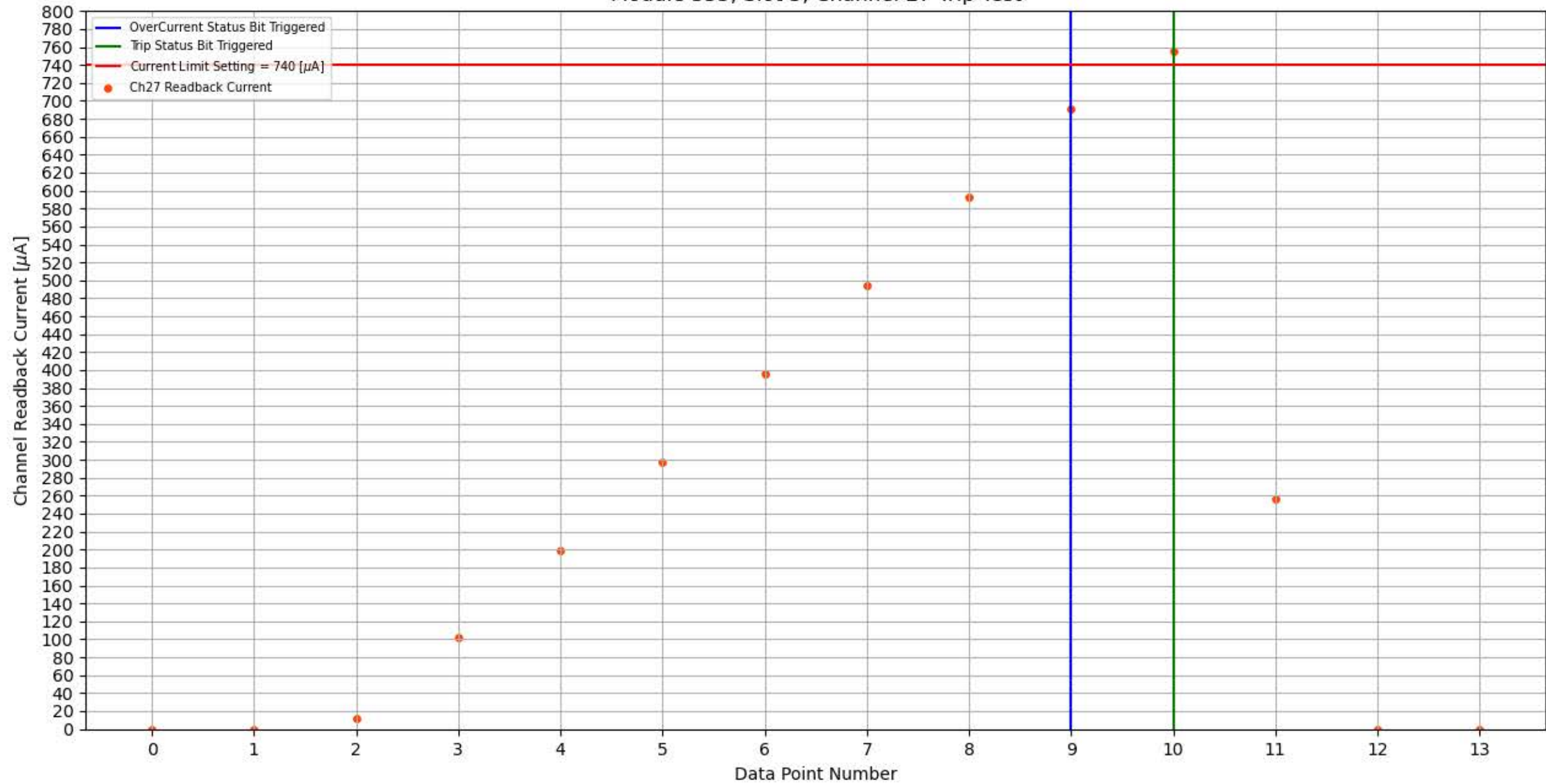
Module 355, Slot 5, Channel 27 Trip Test
