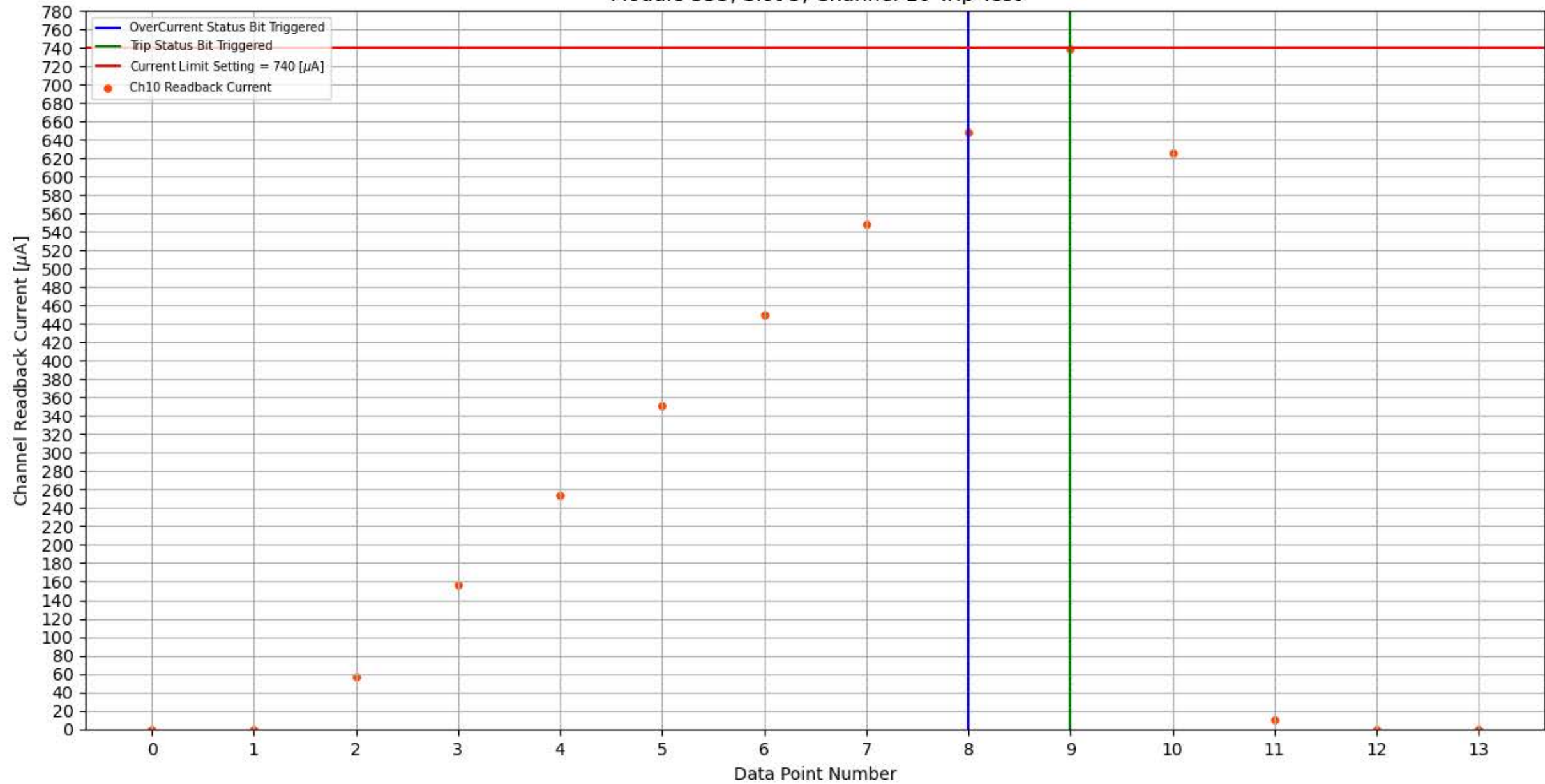
Module 355, Slot 5, Channel 10 Trip Test
