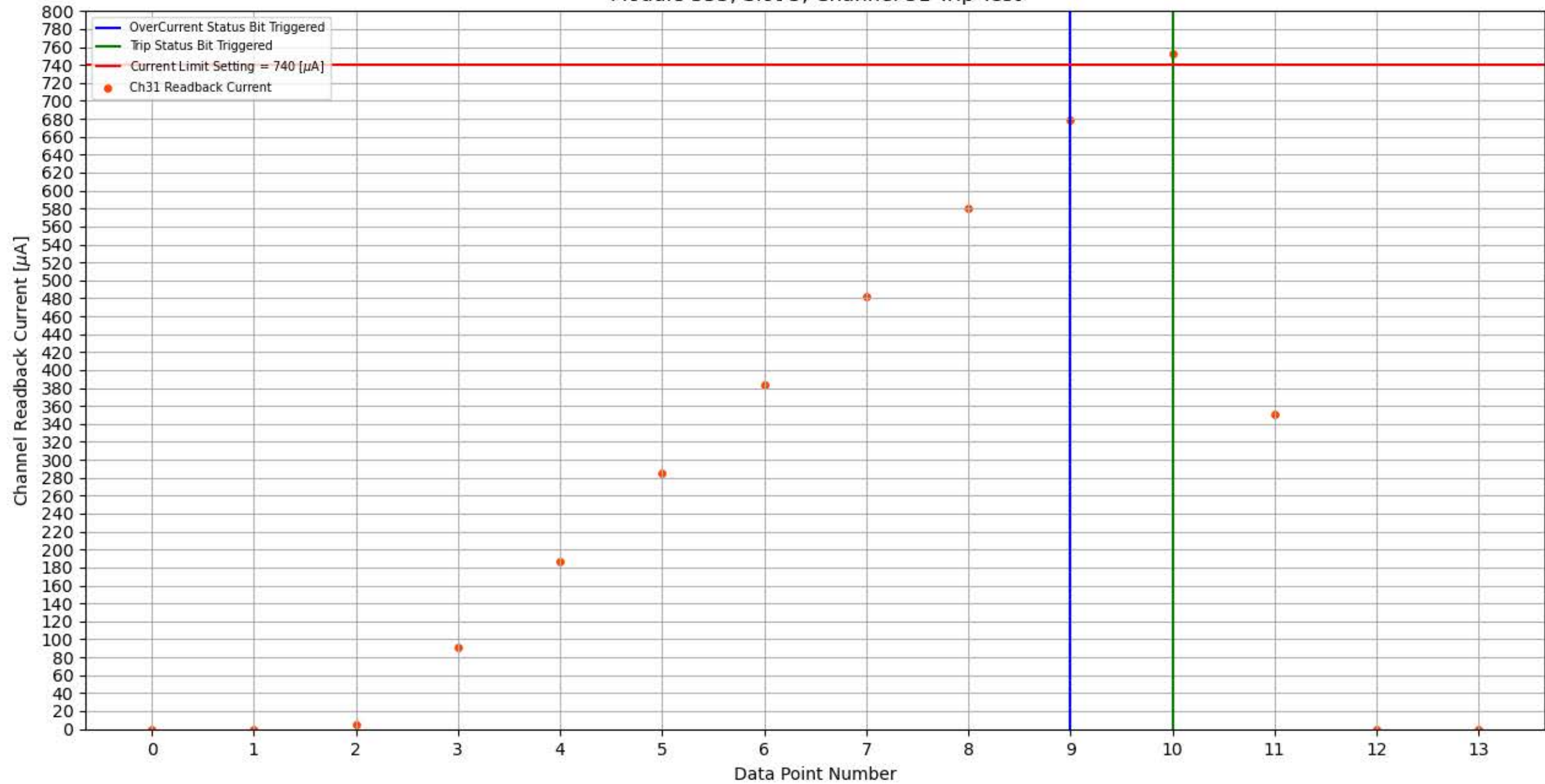
Module 355, Slot 5, Channel 31 Trip Test
