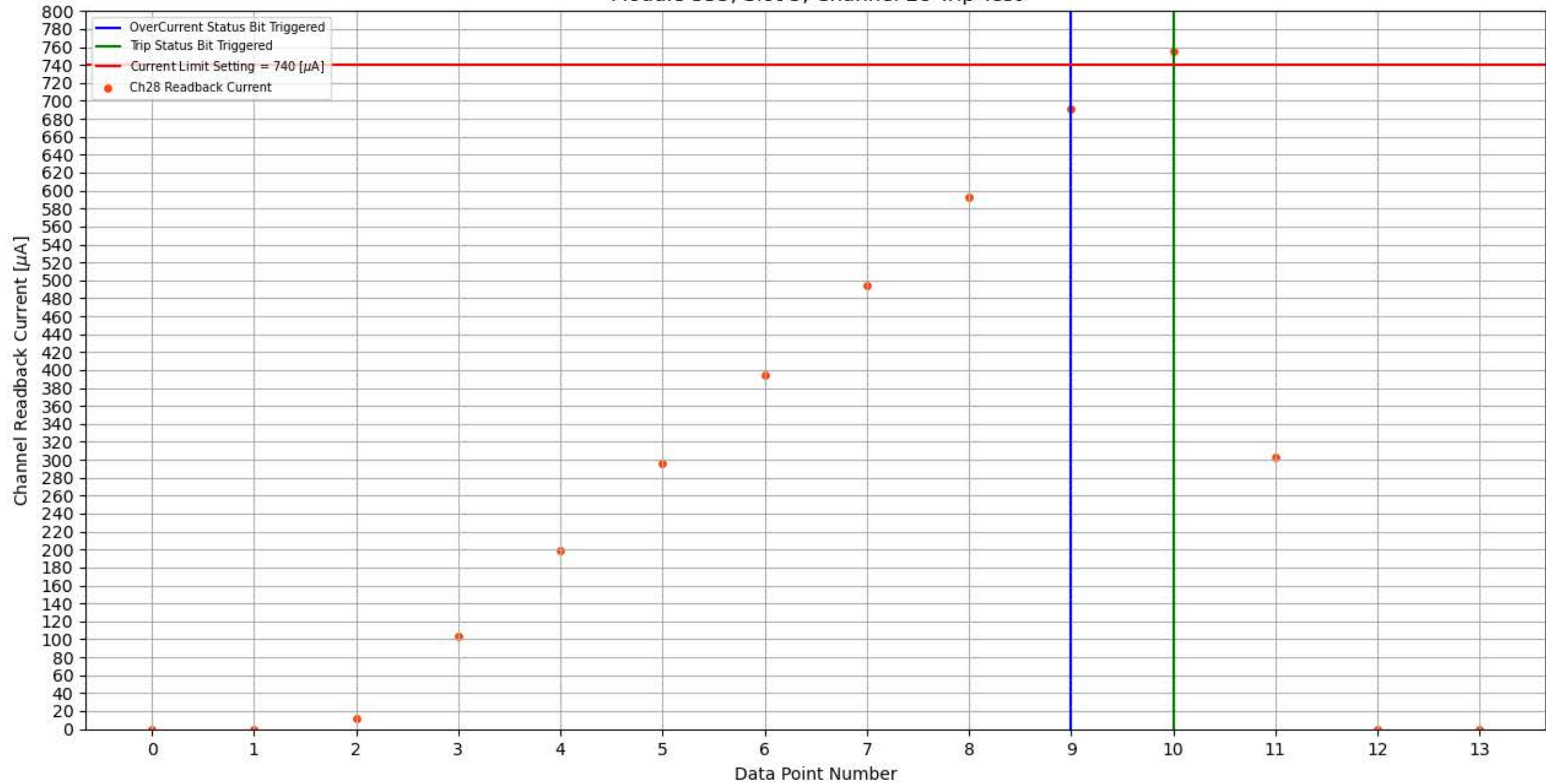
Module 355, Slot 5, Channel 28 Trip Test
