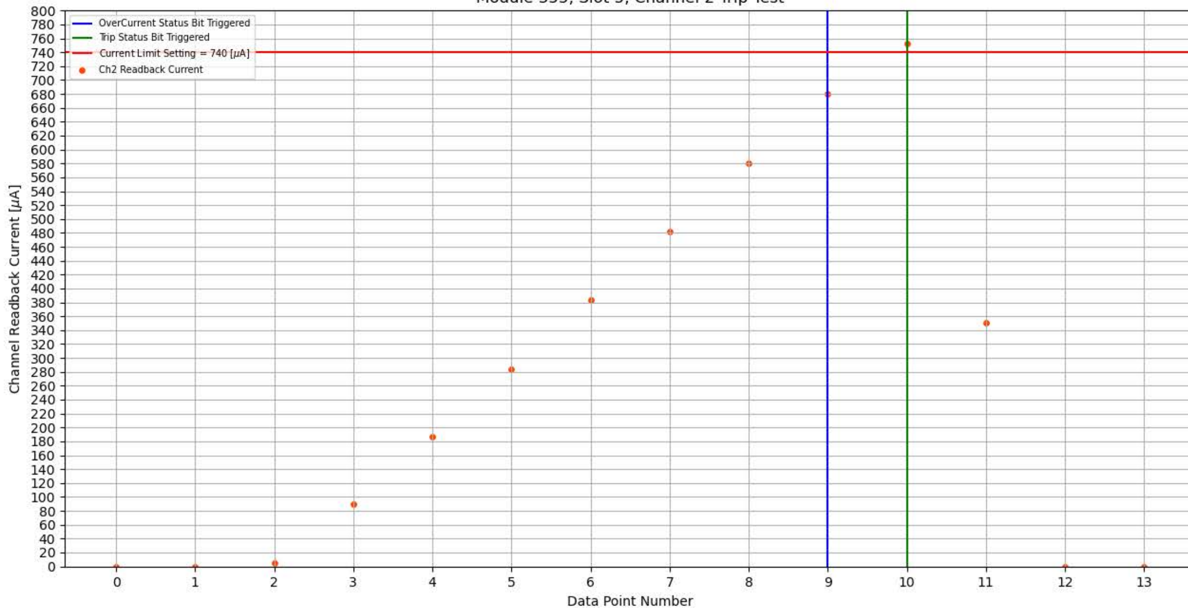
Module 355, Slot 5, Channel 2 Trip Test
