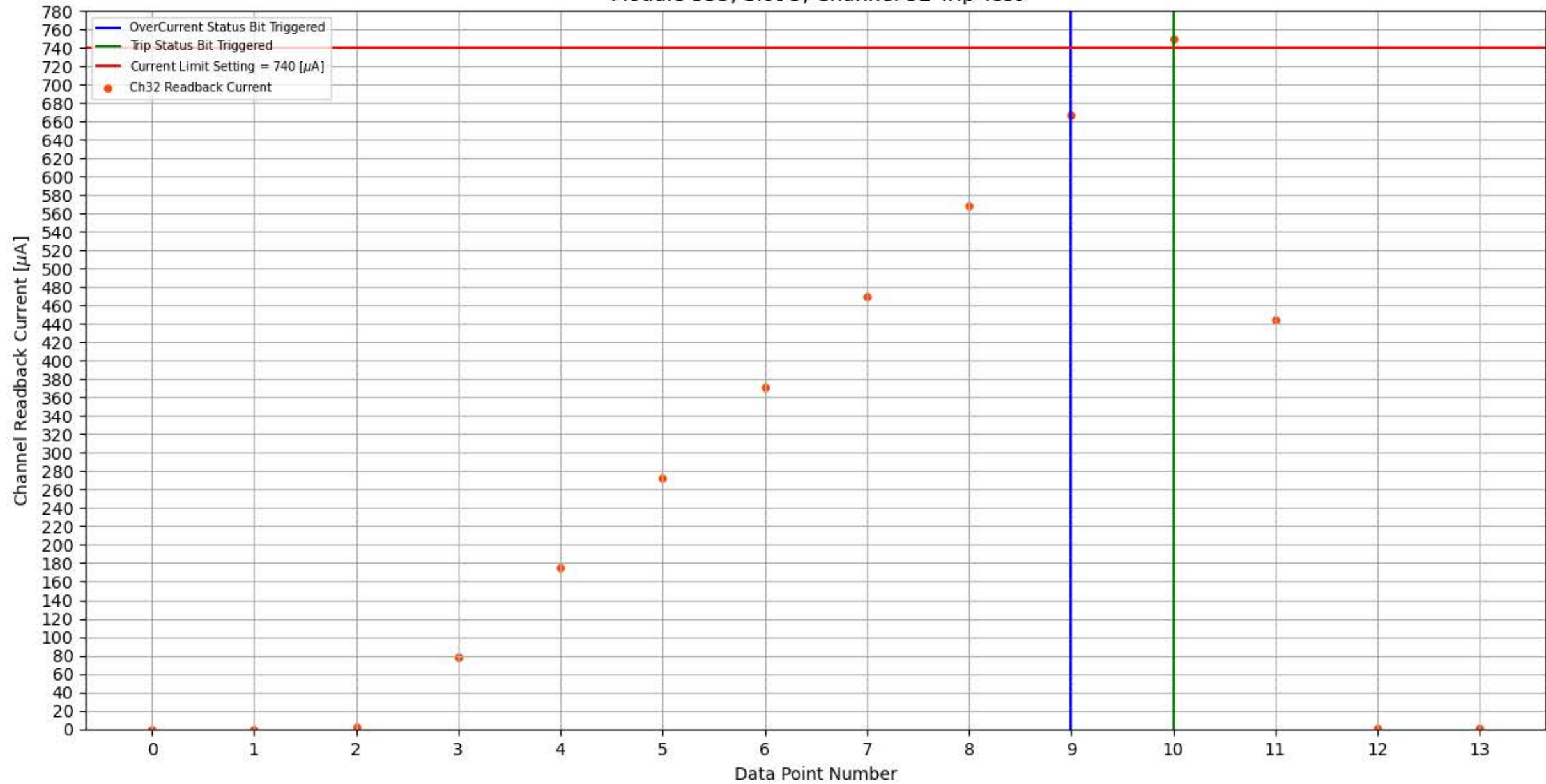
Module 355, Slot 5, Channel 32 Trip Test
