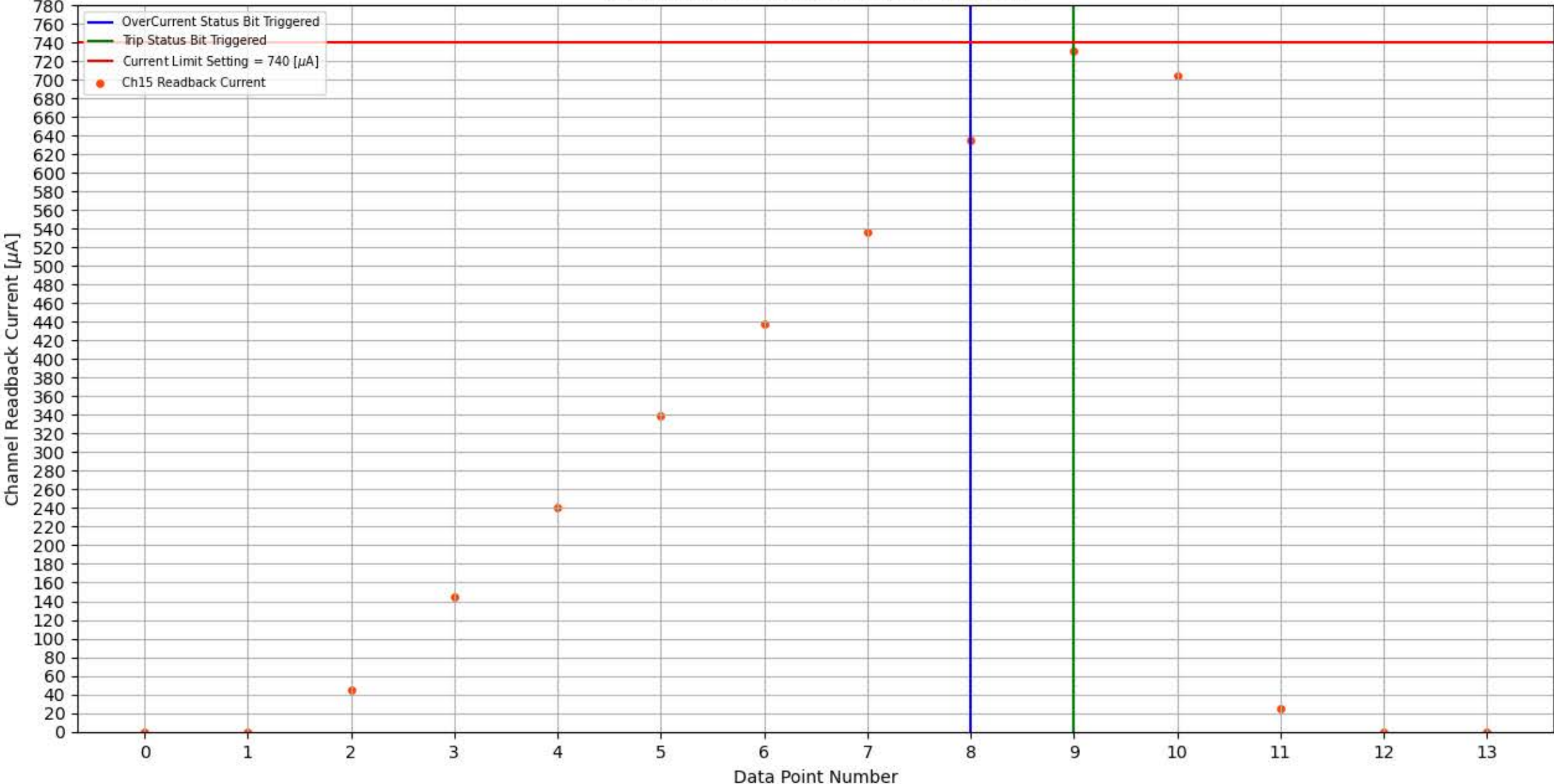
Module 355, Slot 5, Channel 15 Trip Test
