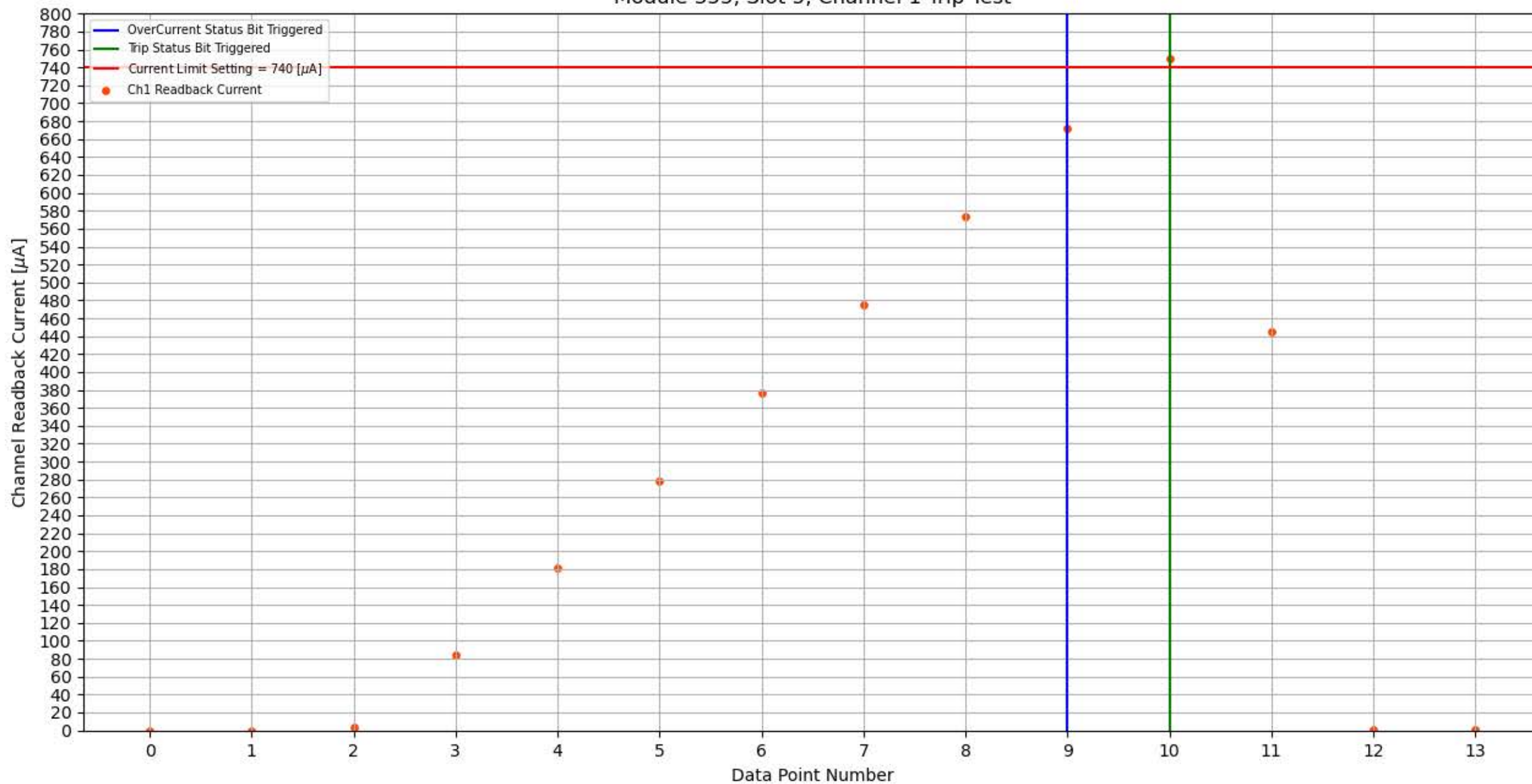
Module 355, Slot 5, Channel 1 Trip Test
