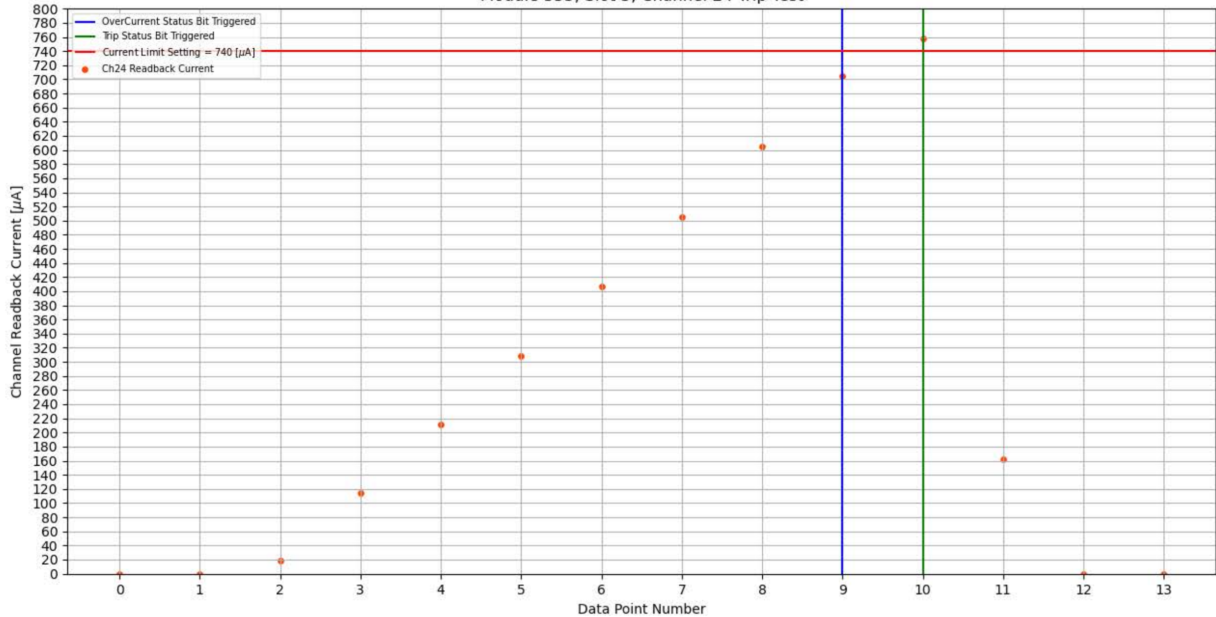
Module 355, Slot 5, Channel 24 Trip Test
