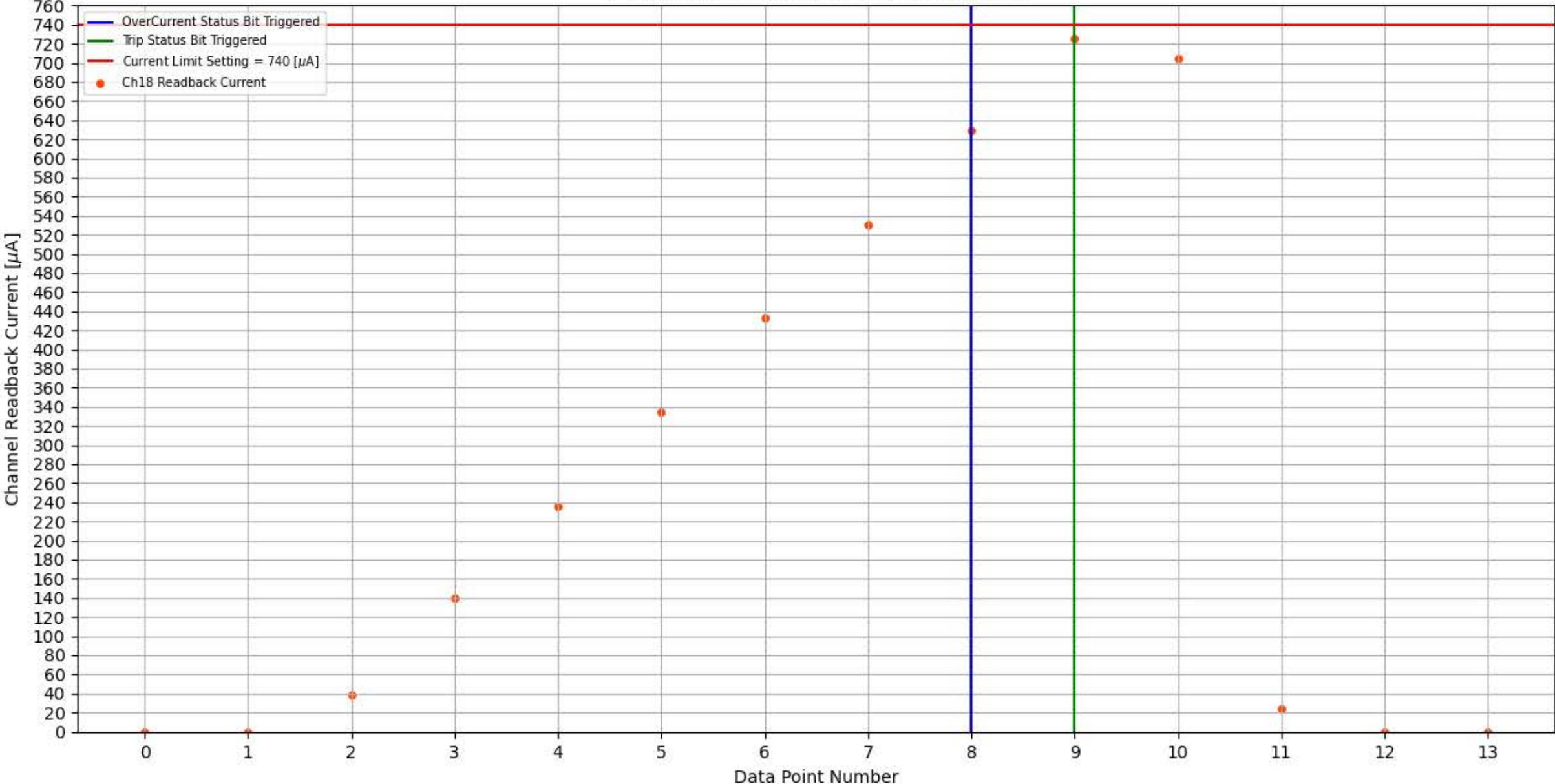
Module 355, Slot 5, Channel 18 Trip Test
