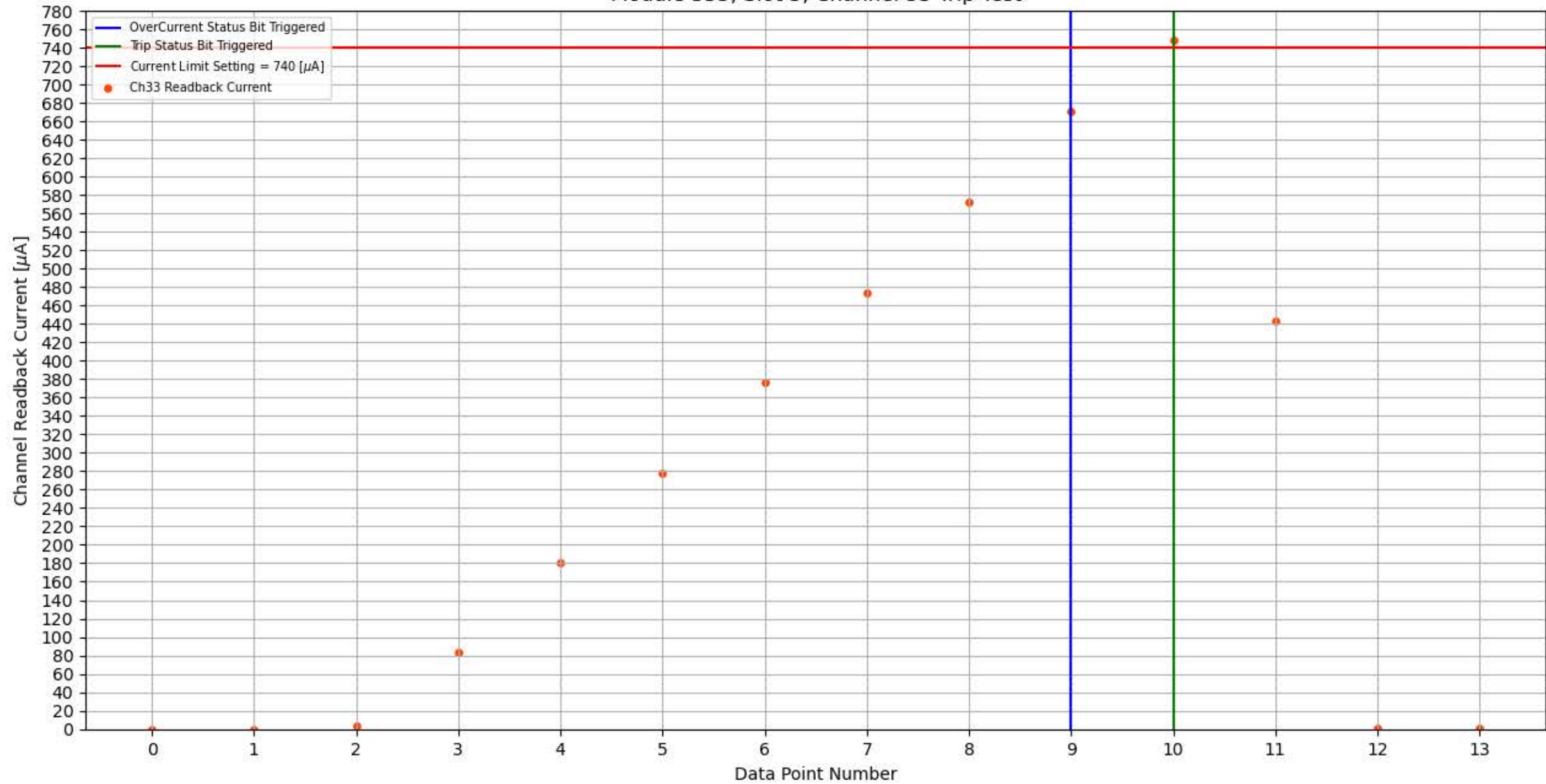
Module 355, Slot 5, Channel 33 Trip Test
