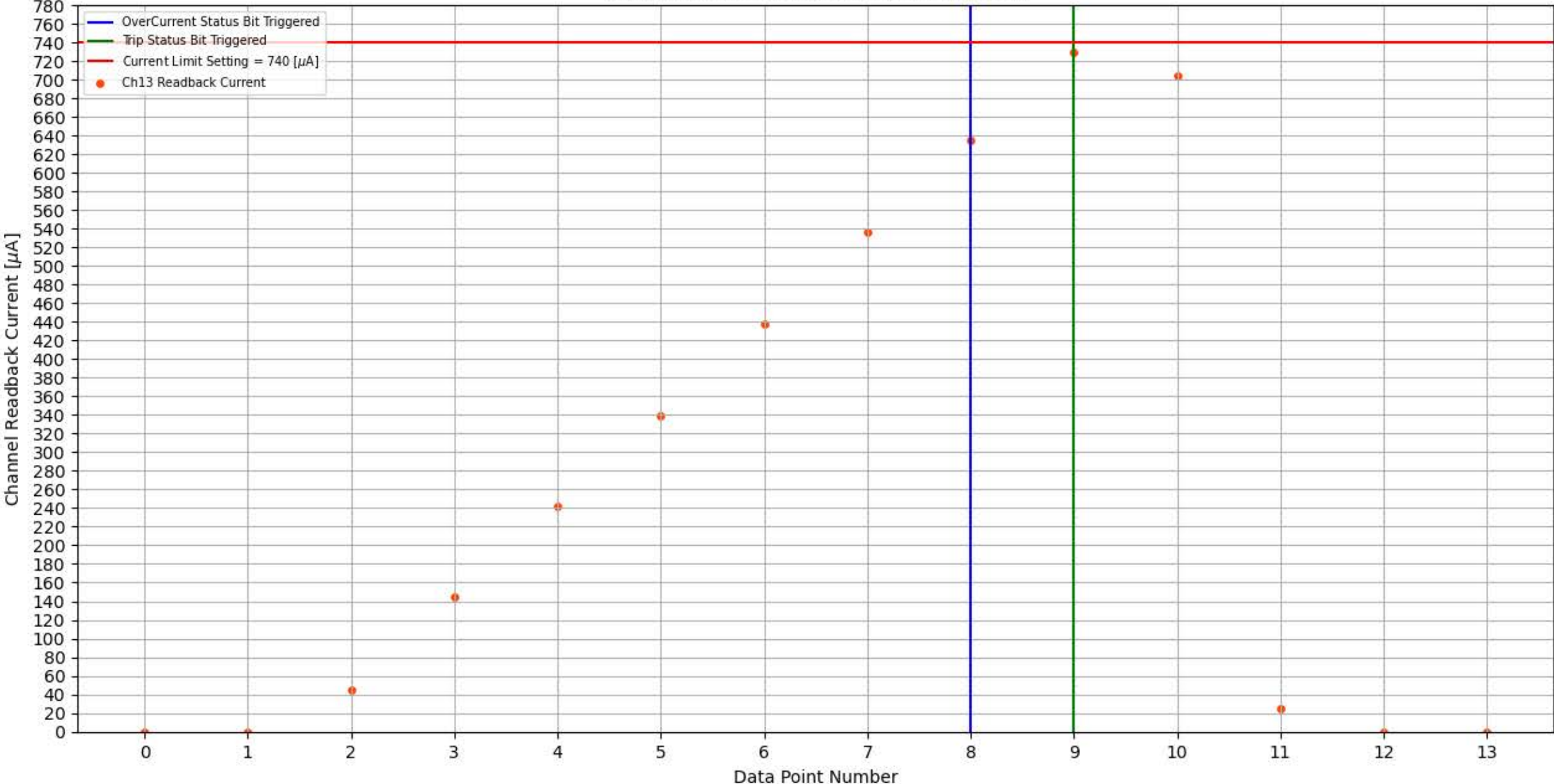
Module 355, Slot 5, Channel 13 Trip Test
