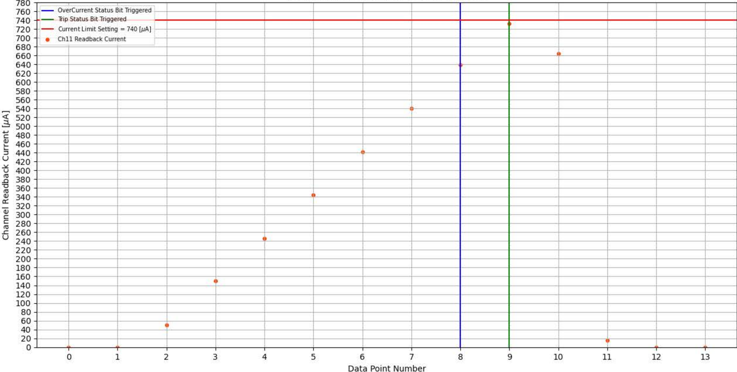
Module 355, Slot 5, Channel 11 Trip Test
