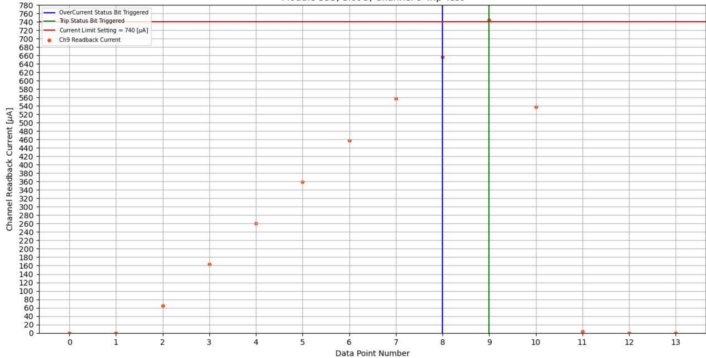
Module 355, Slot 5, Channel 9 Trip Test
