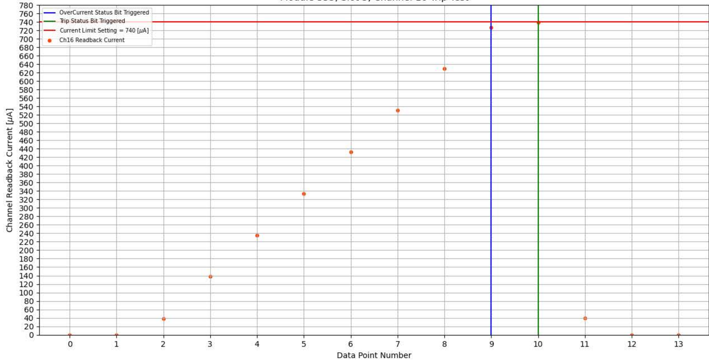
Module 355, Slot 5, Channel 16 Trip Test
