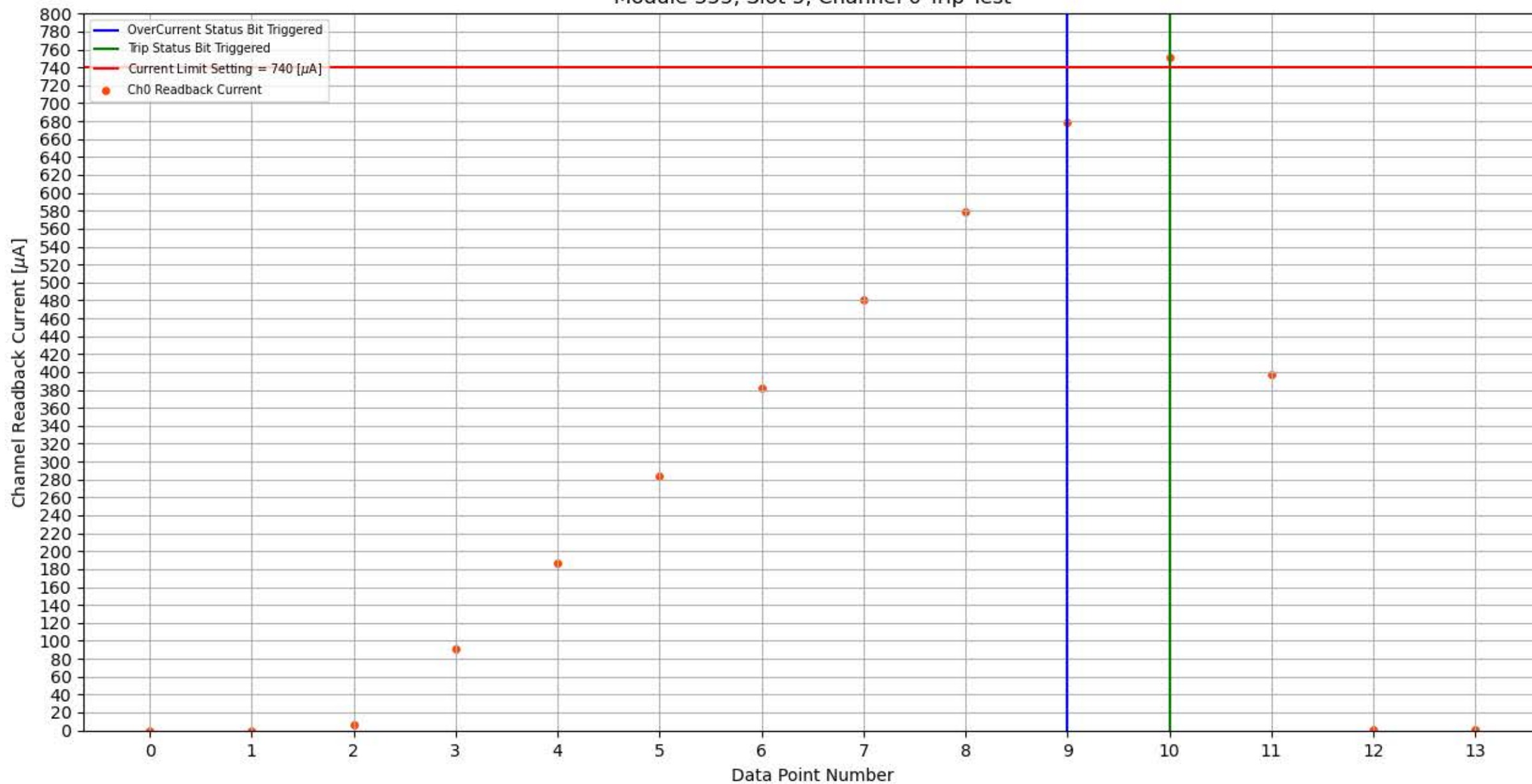
Module 355, Slot 5, Channel 0 Trip Test
