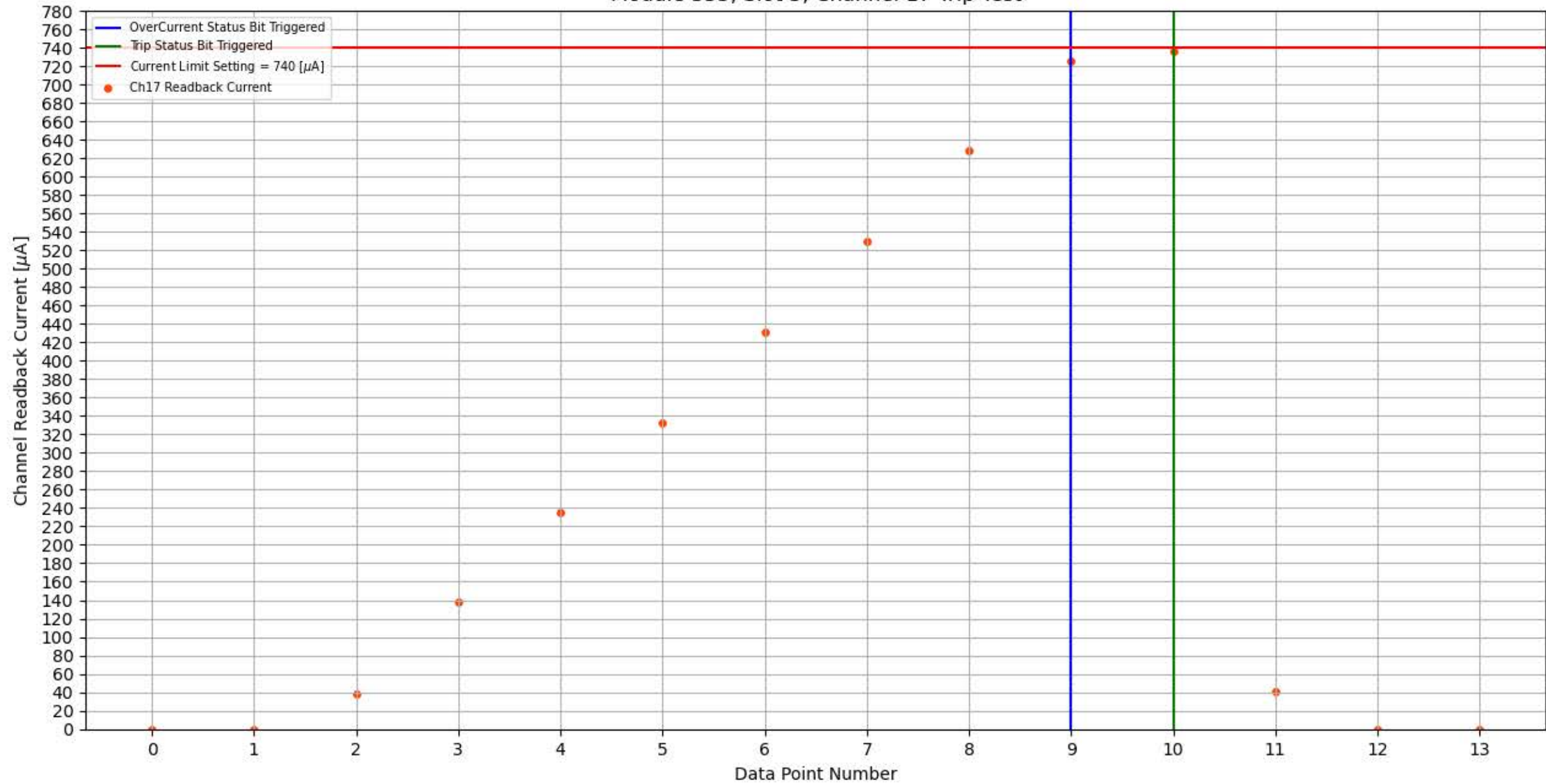
Module 355, Slot 5, Channel 17 Trip Test
