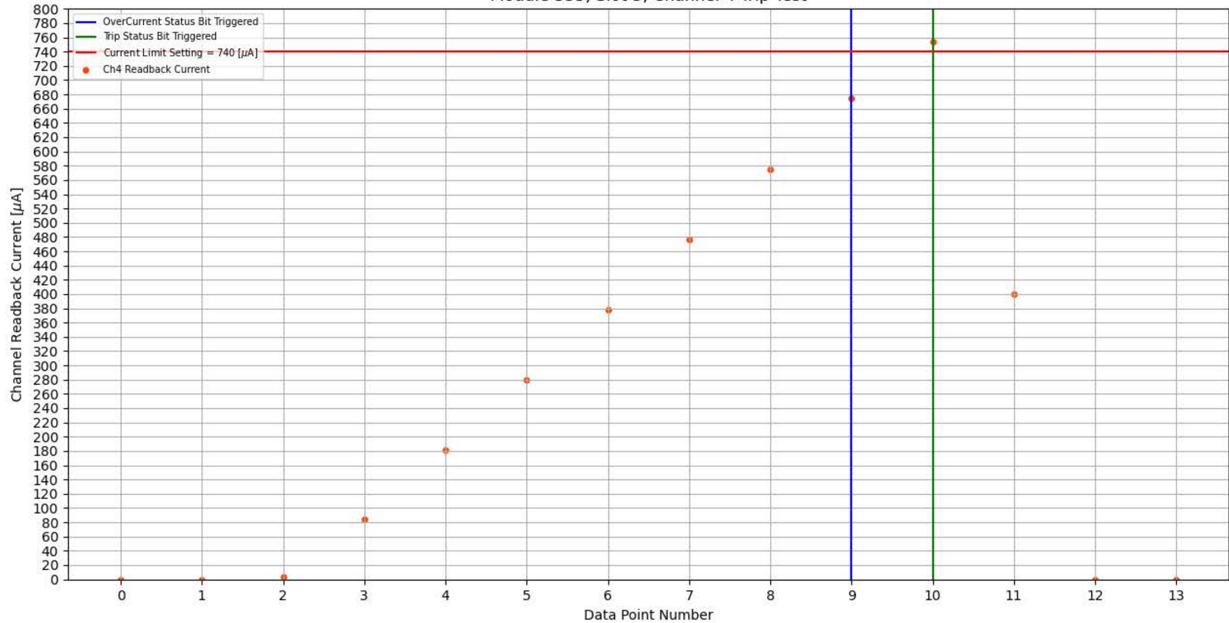
Module 355, Slot 5, Channel 4 Trip Test
