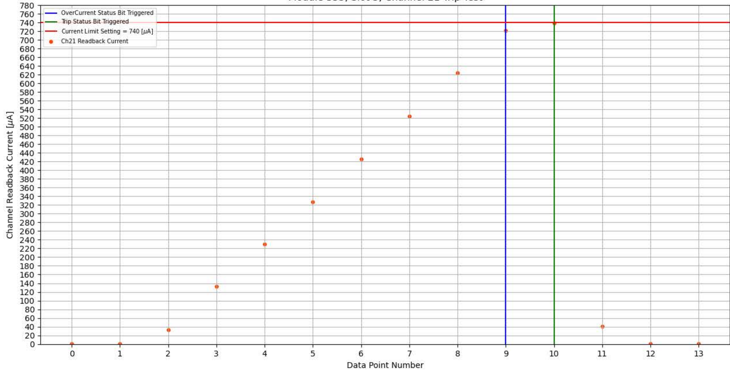
Module 355, Slot 5, Channel 21 Trip Test
