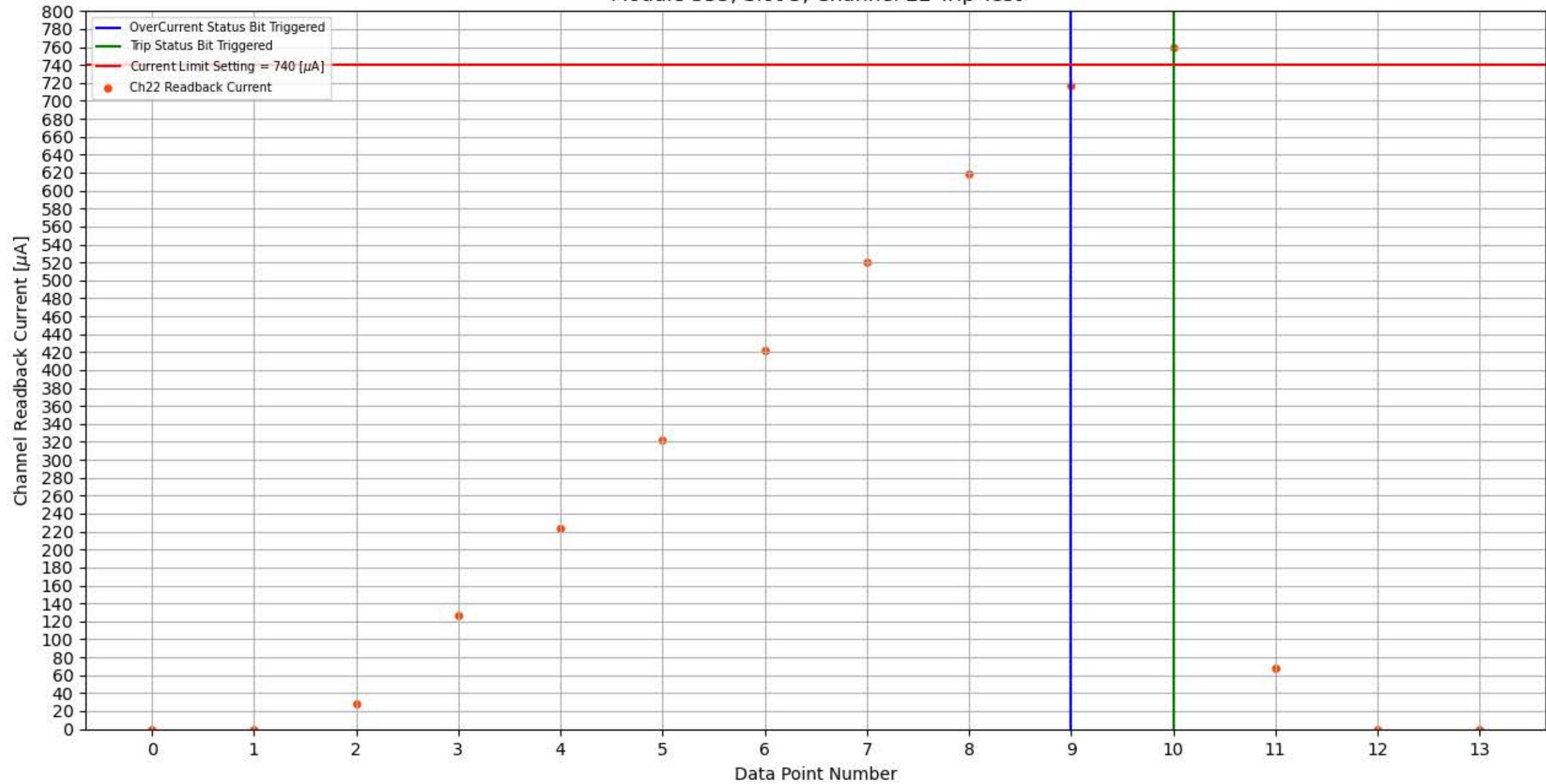
Module 355, Slot 5, Channel 22 Trip Test
