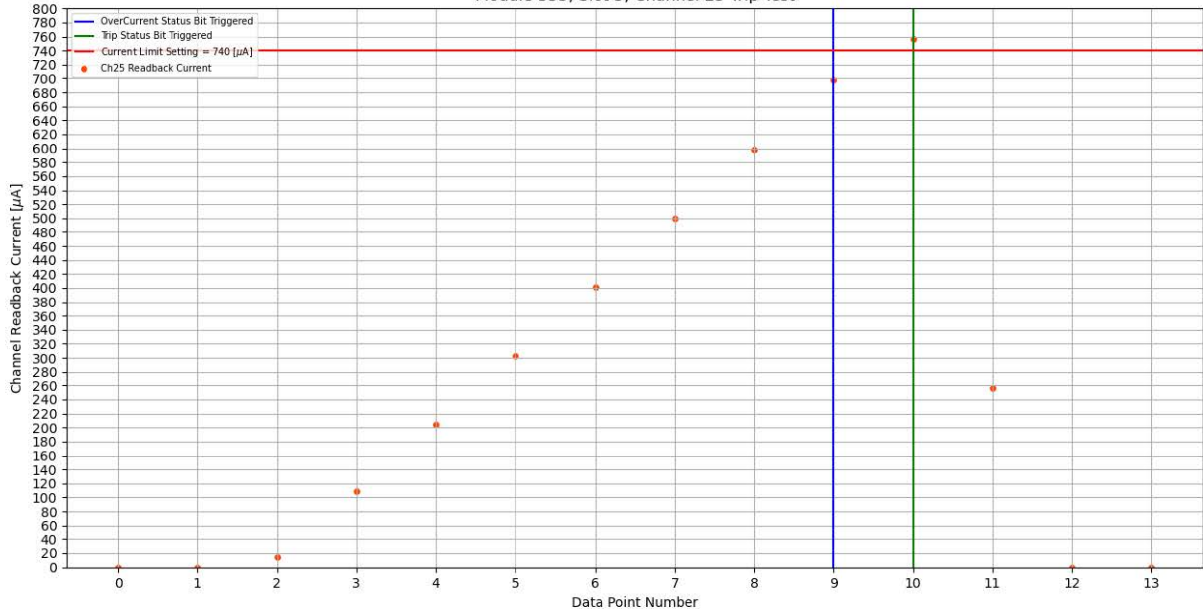
Module 355, Slot 5, Channel 25 Trip Test
