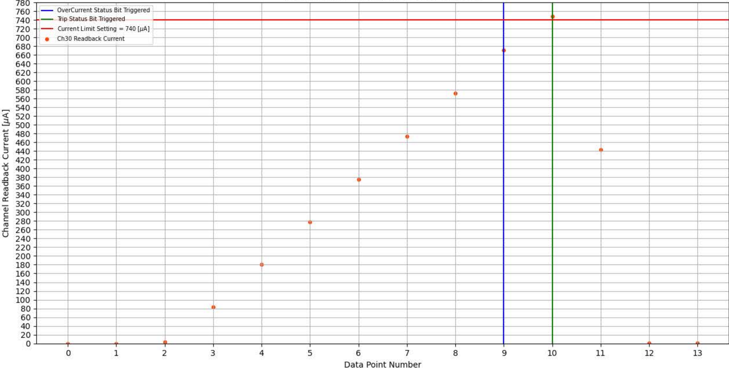
Module 355, Slot 5, Channel 30 Trip Test
