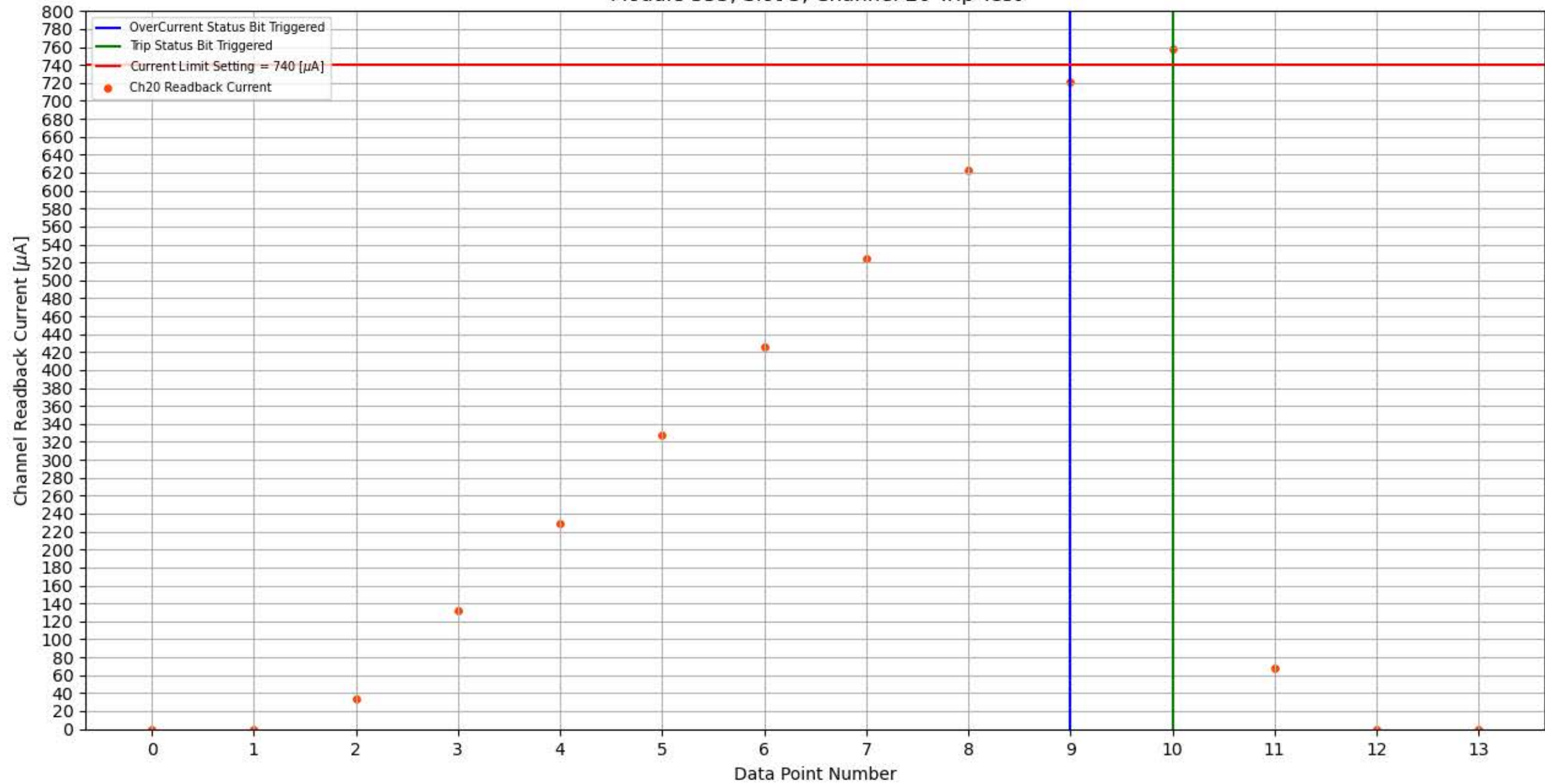
Module 355, Slot 5, Channel 20 Trip Test
