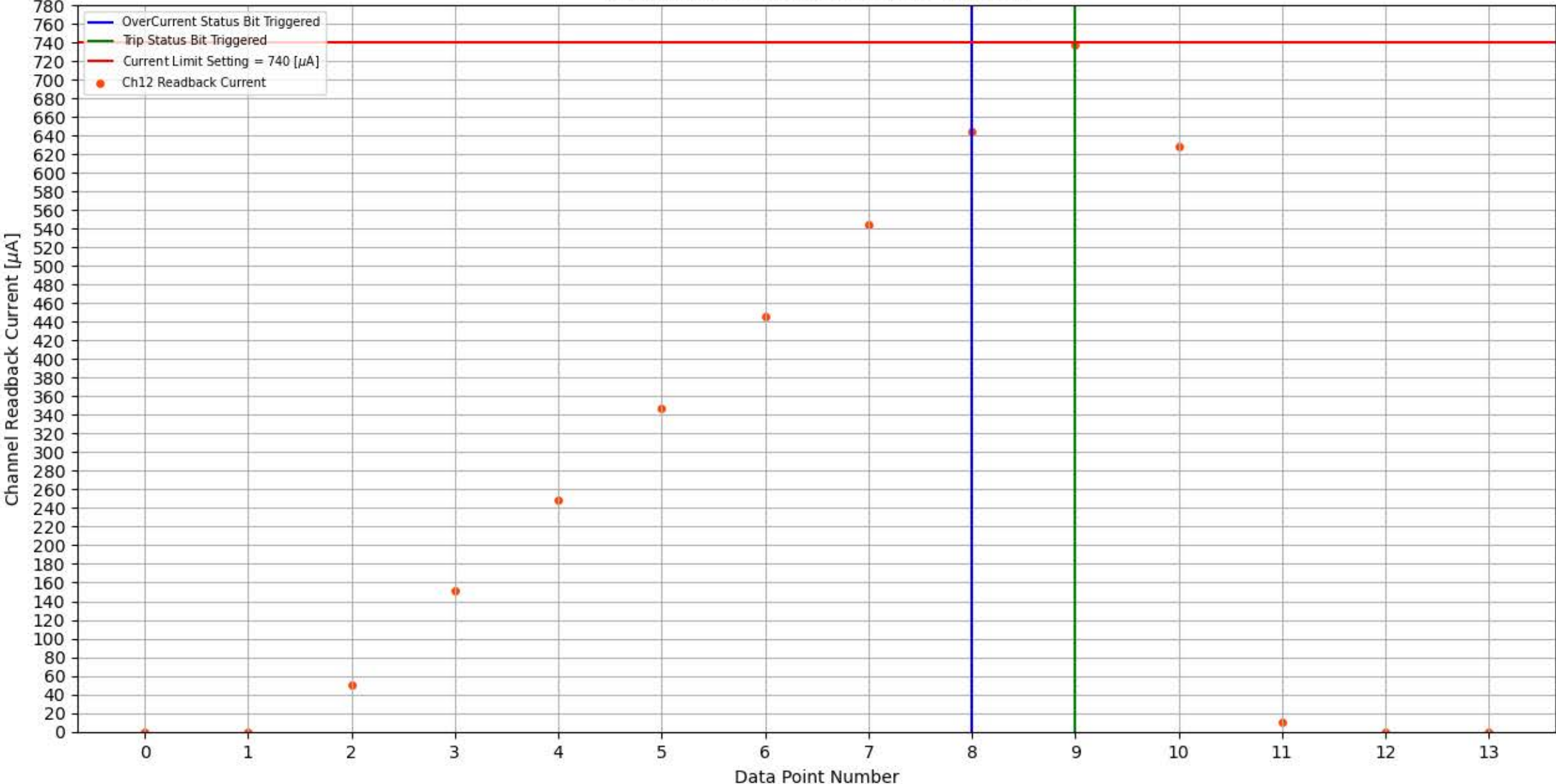
Module 355, Slot 5, Channel 12 Trip Test
