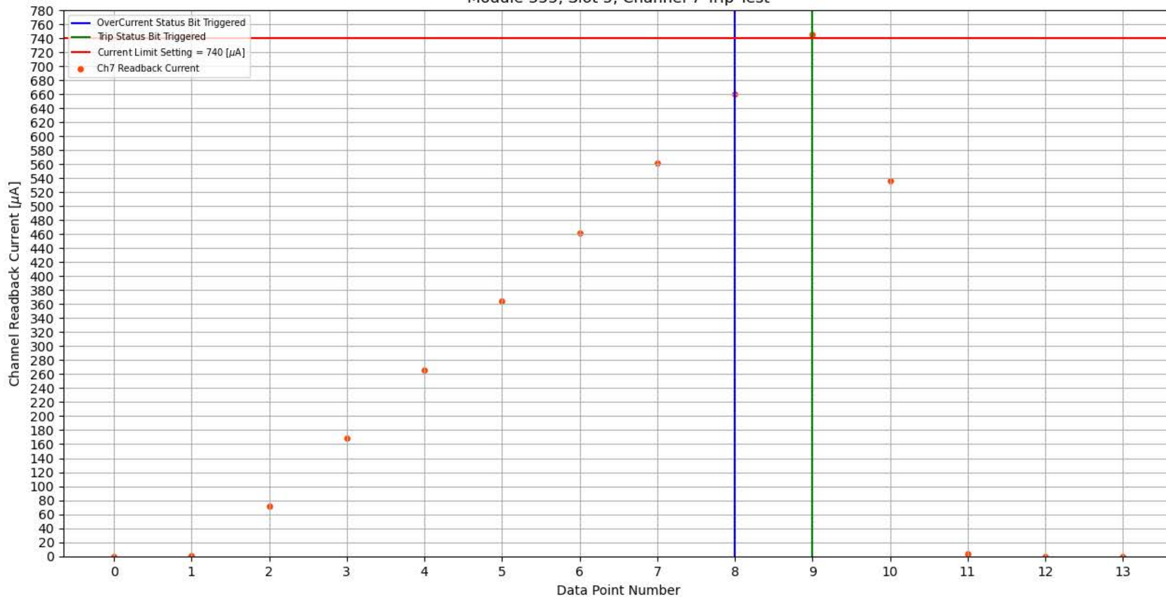
Module 355, Slot 5, Channel 7 Trip Test
