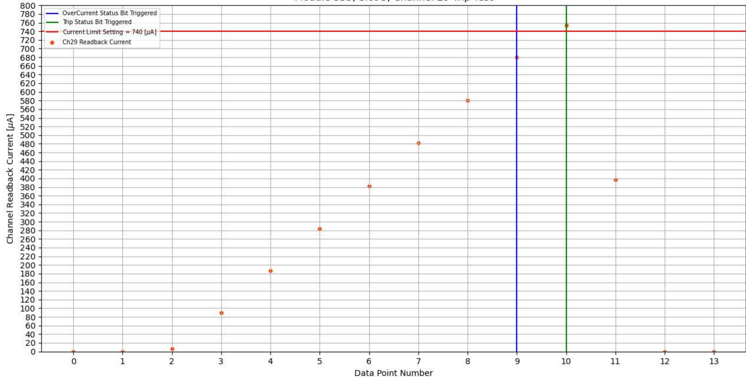
Module 355, Slot 5, Channel 29 Trip Test
