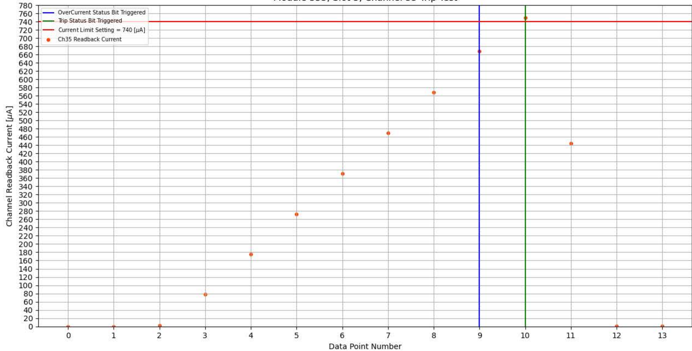
Module 355, Slot 5, Channel 35 Trip Test
