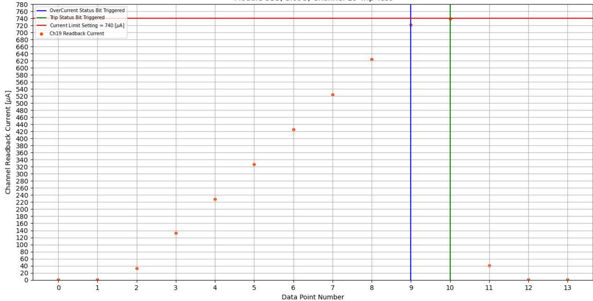
Module 355, Slot 5, Channel 19 Trip Test
