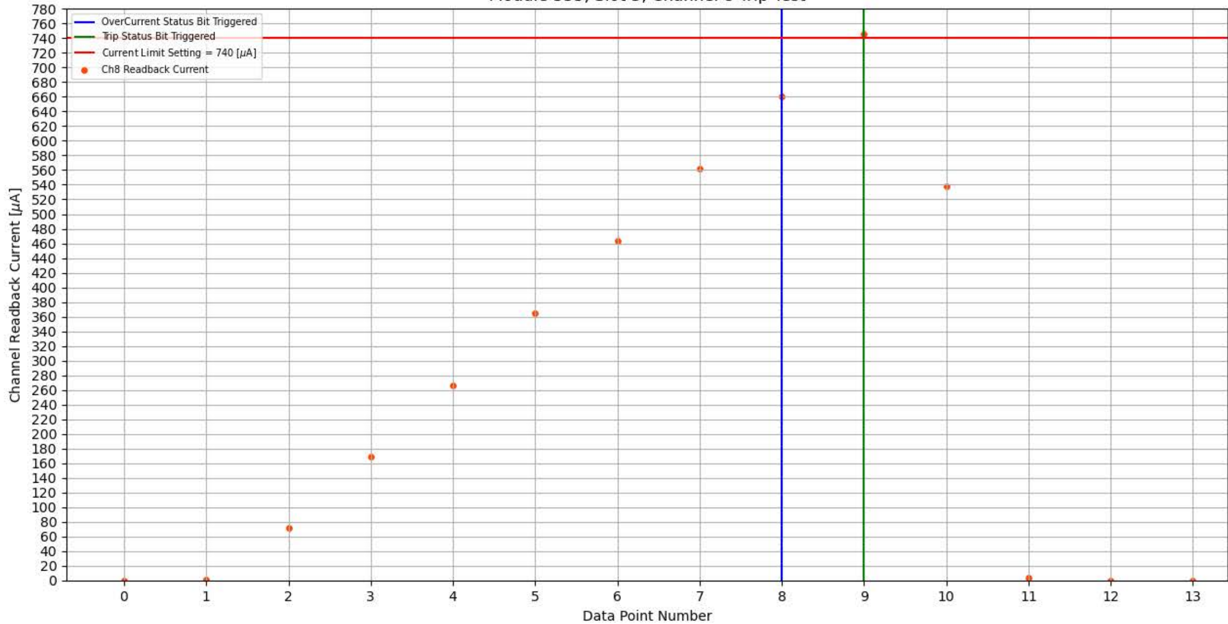
Module 355, Slot 5, Channel 8 Trip Test
