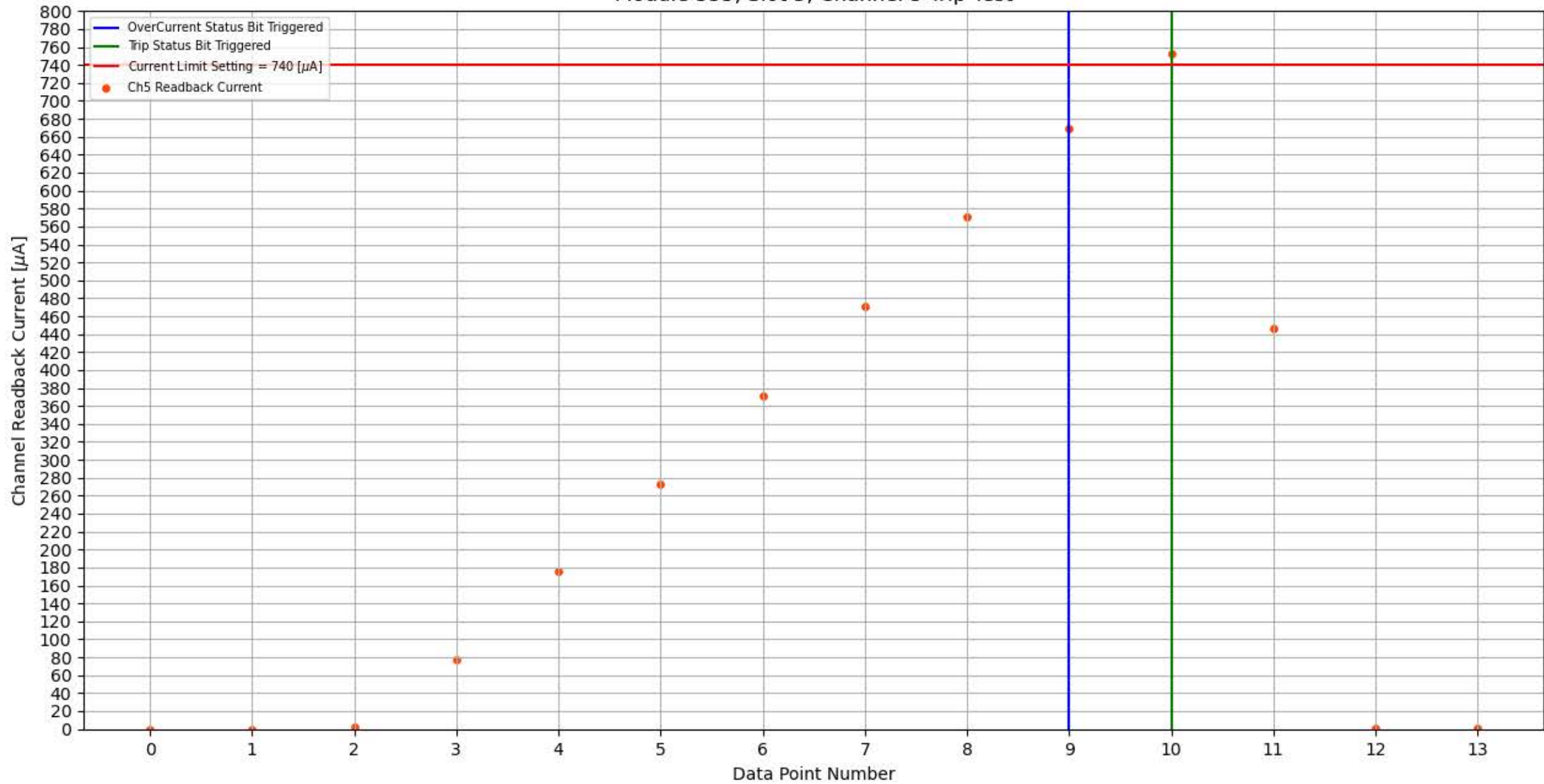
Module 355, Slot 5, Channel 5 Trip Test
