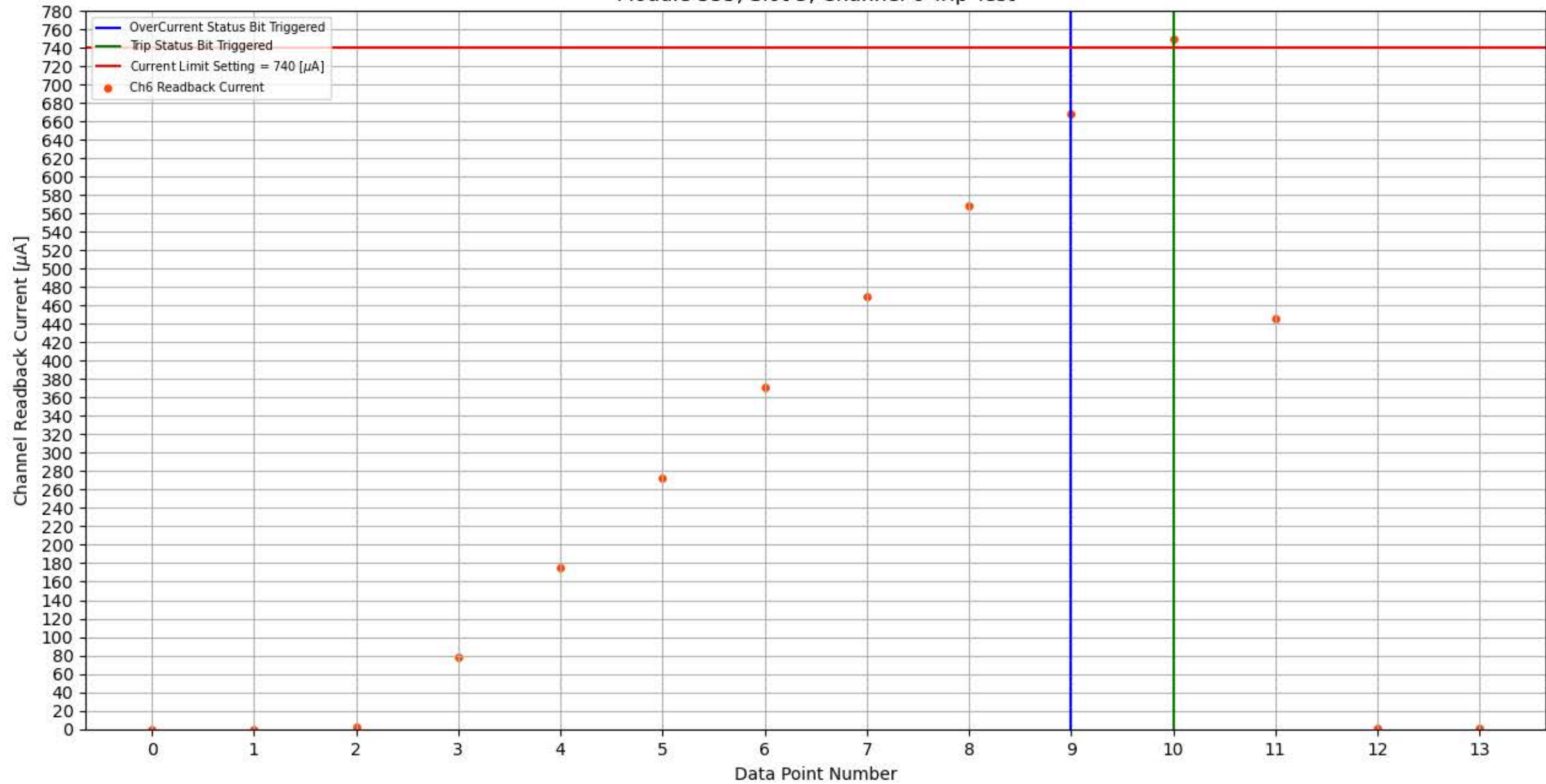
Module 355, Slot 5, Channel 6 Trip Test
