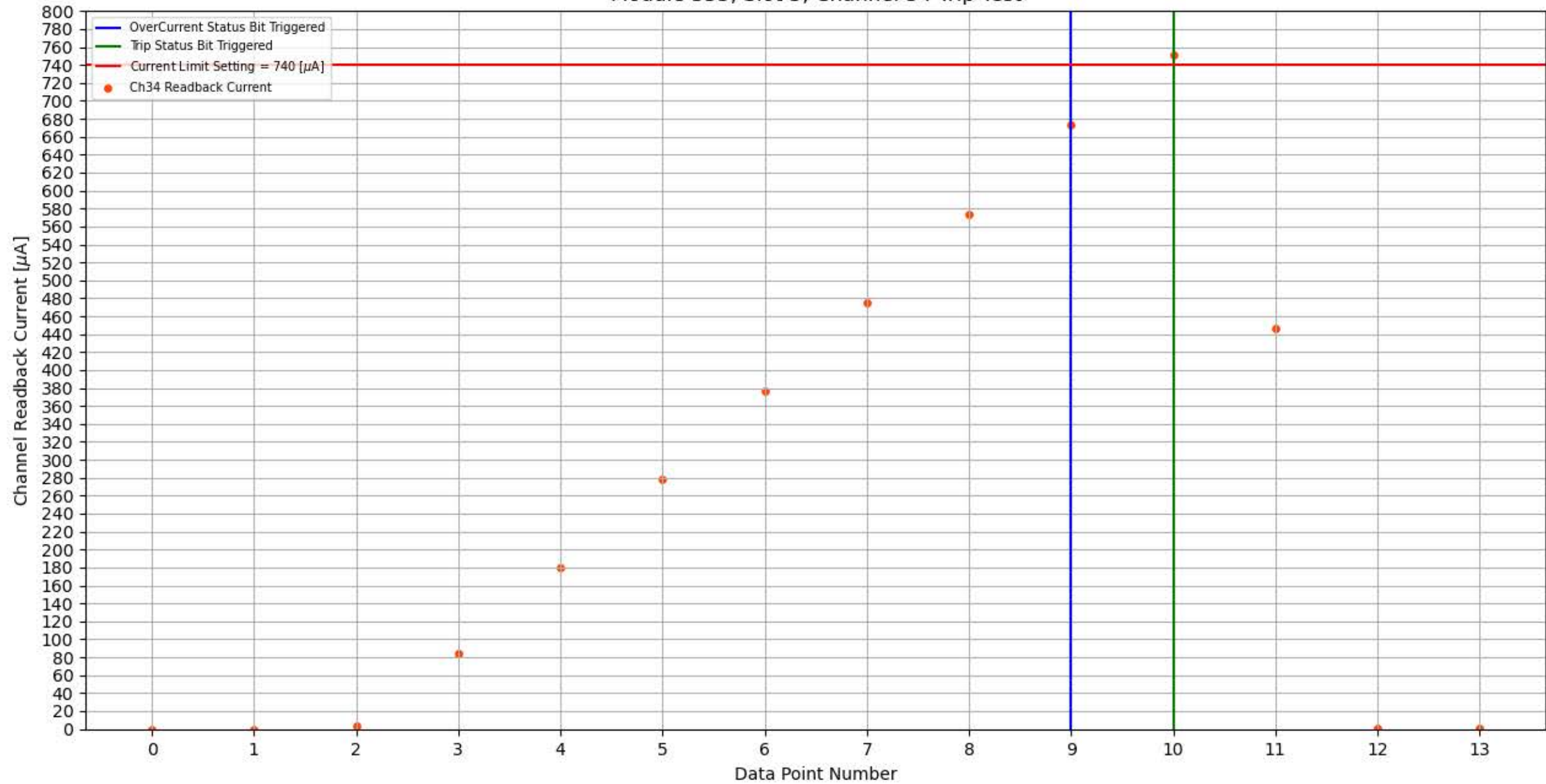
Module 355, Slot 5, Channel 34 Trip Test
