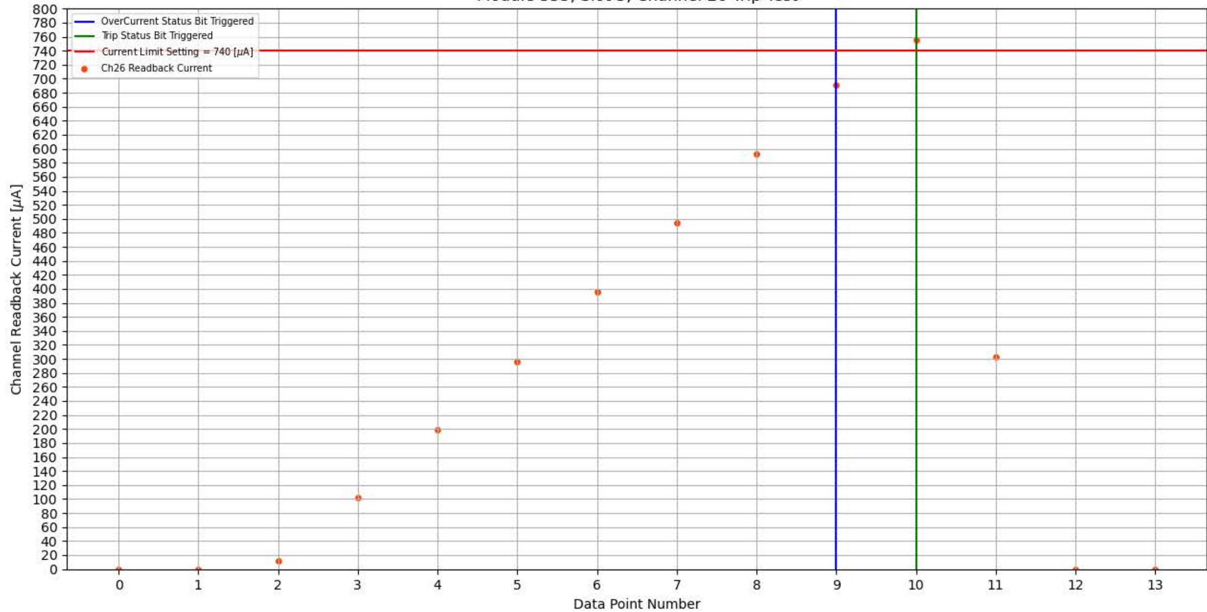
Module 355, Slot 5, Channel 26 Trip Test
